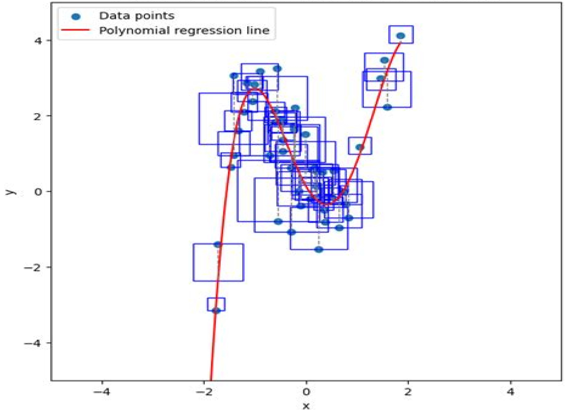
Polynomial (degree = 4) regression with residuals
